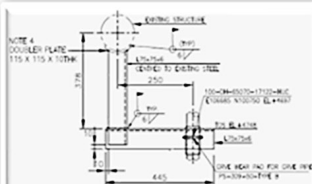
PSA-HLIC-0008A Pipe Support Detail
